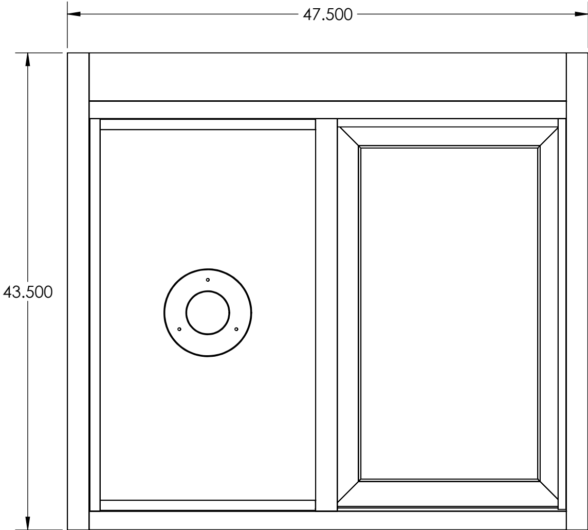
MODEL 600 47.5"W X 43.5"H R/L FROM EXTERIOR VIEW LEXAN SPEAK THRU IN FIXED PANE
