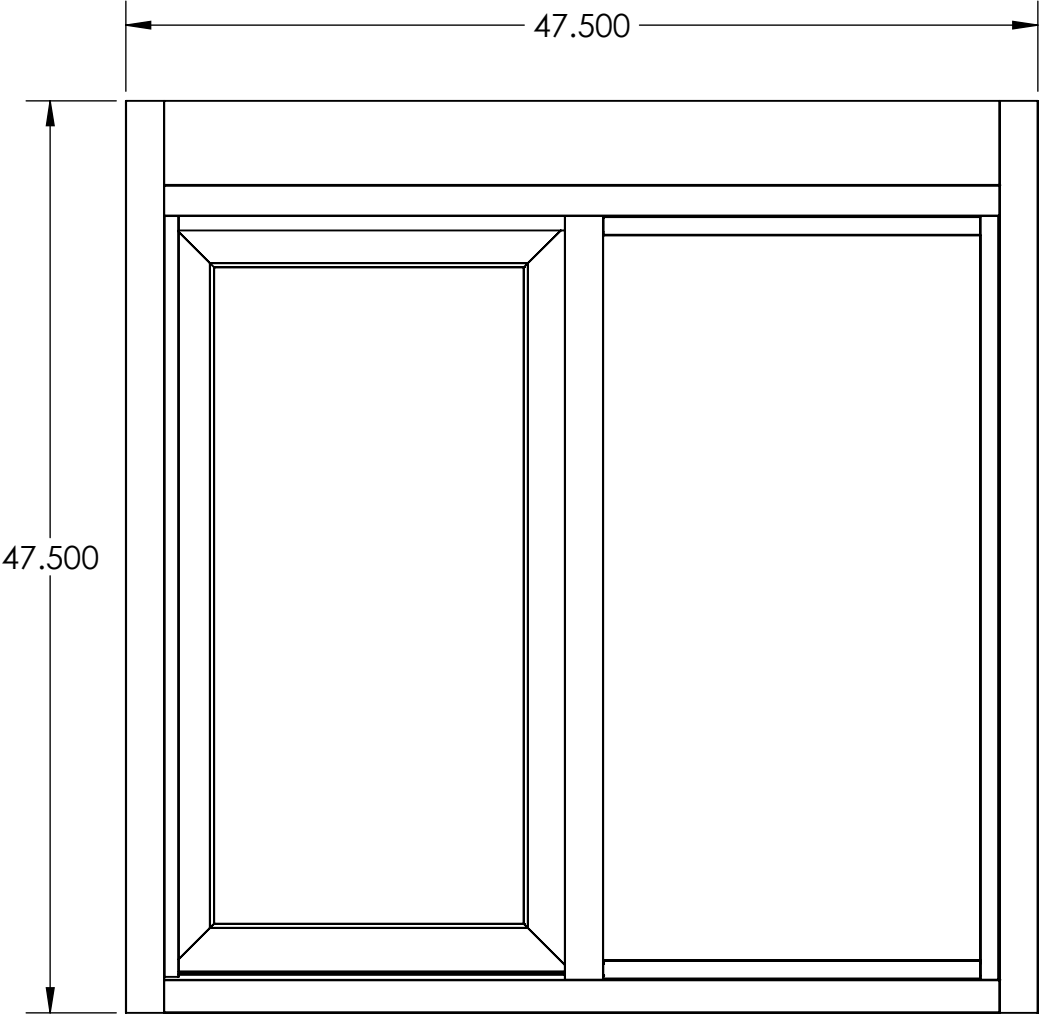
MODEL 600 L/R DIRECTION FROM OUTSIDE VIEW
