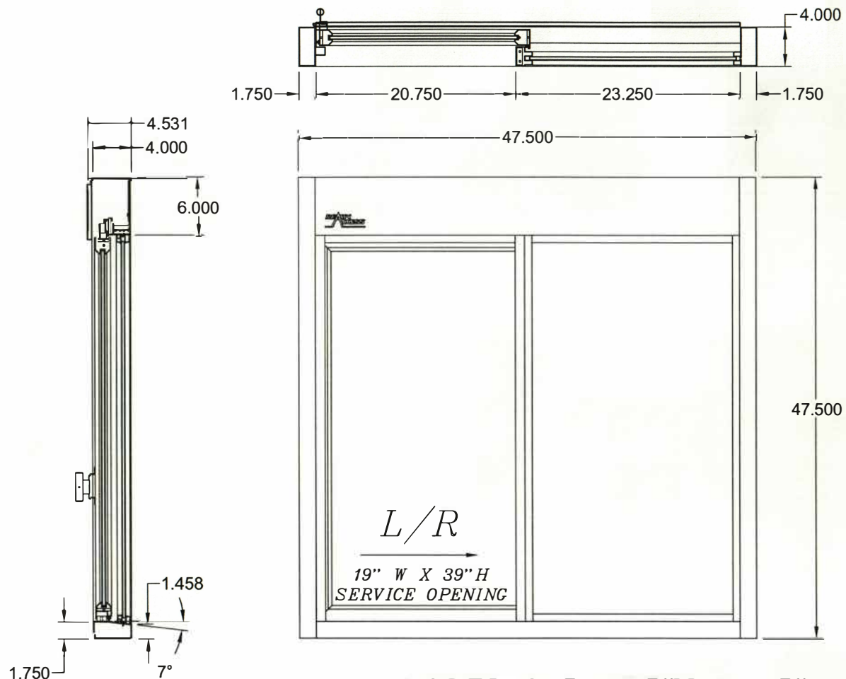
MODEL 275 47.5"W X 47.5"H L/R DIRECTION FROM OUTSIDE VIEW
