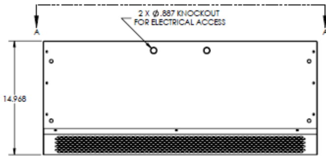
RAC-36 FRONT VIEW
