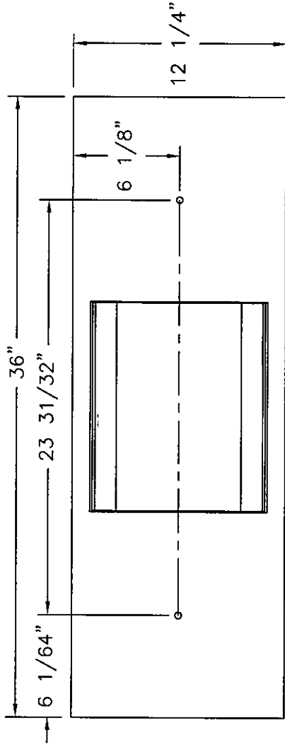
TOP VIEW
