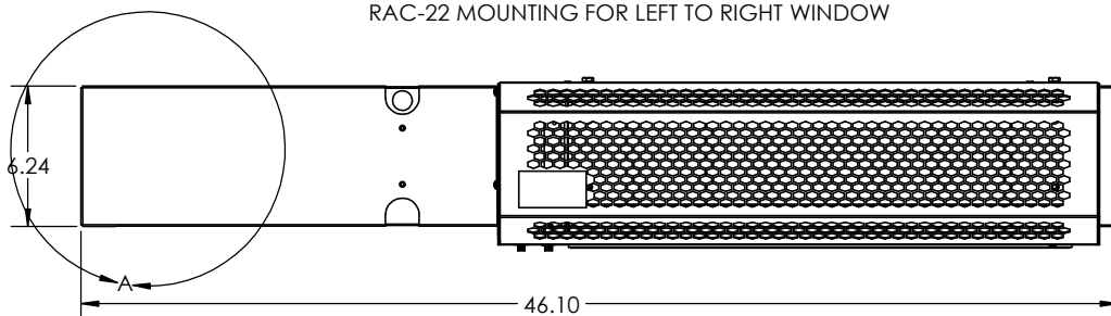
RAC-22 MOUNTING FOR LEFT TO RIGHT WINDOW
