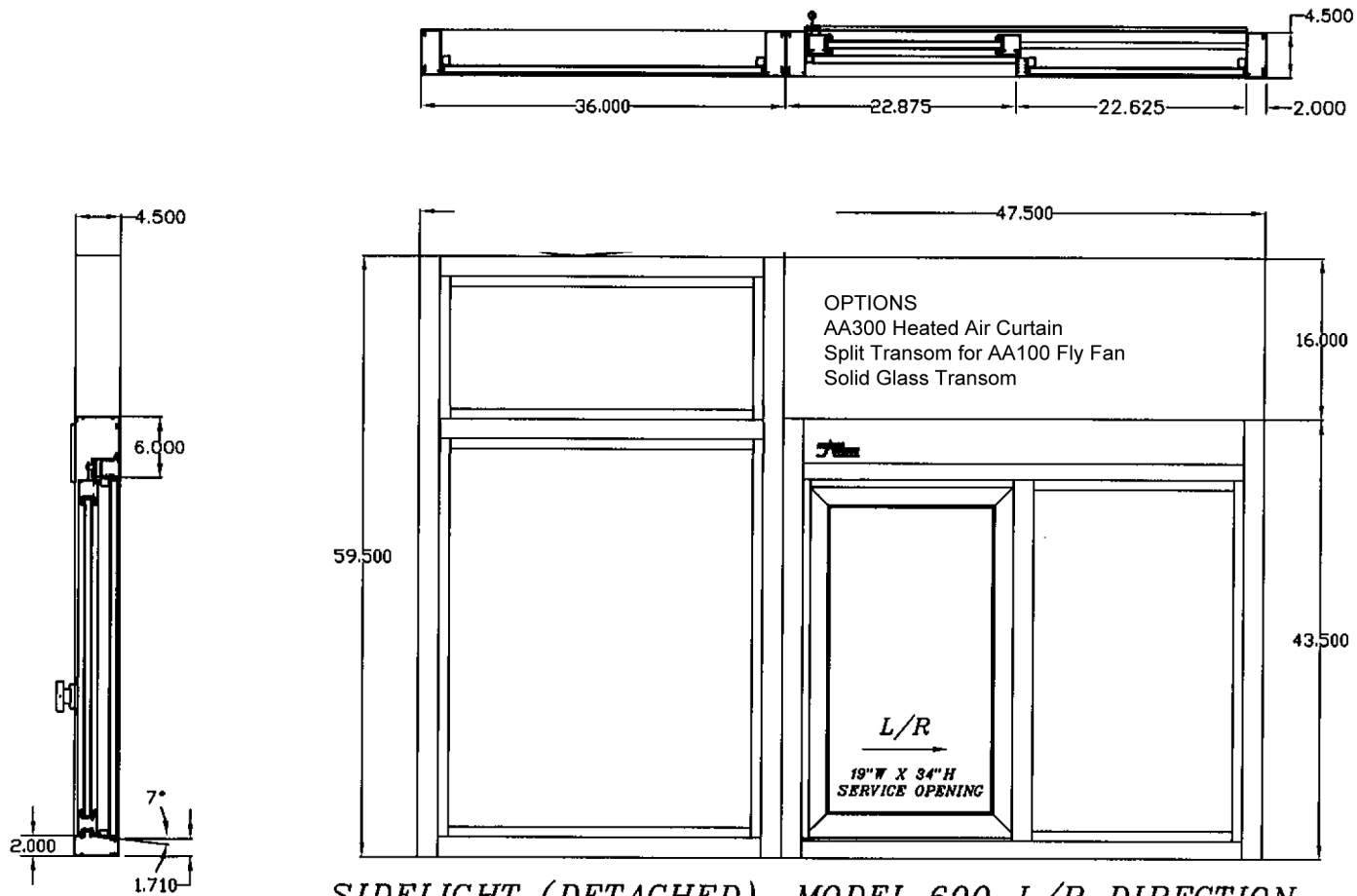
SIDELIGHT (DETACHED) MODEL 600 L/R DIRECTION FROM OUTSIDE VIEW.
