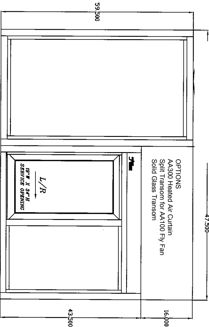
SIDELIGHT (DETACHED)
