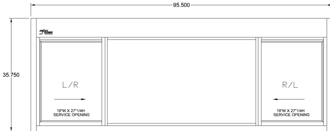
Model 650 - 95 1/2 X 35 3/4H OUTSIDE VIEW
