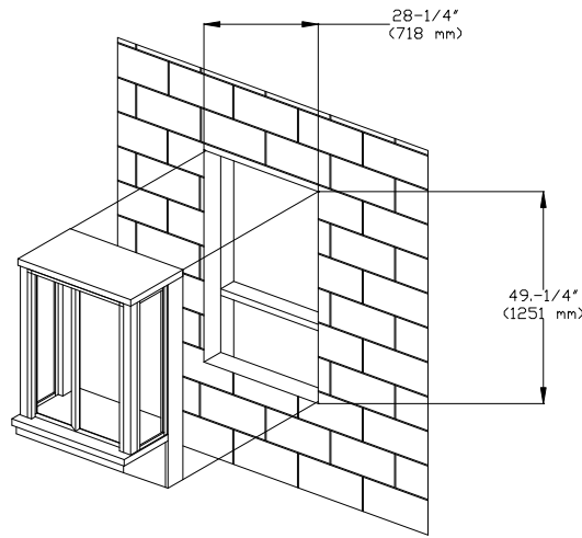
MASONRY WALL ROUGH OPENING
