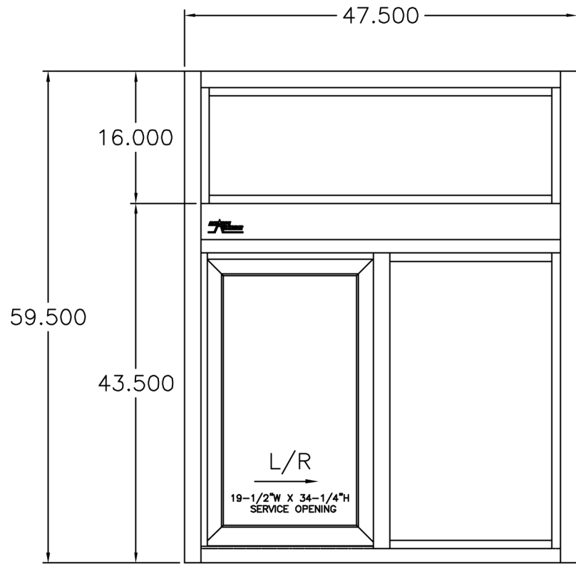
MODEL 600 WITH 16" ATTACHED TRANSOM L/R DIRECTION FROM OUTSIDE VIEW
